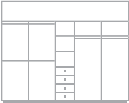
5 Door – 2400mm H x 3000mm W
