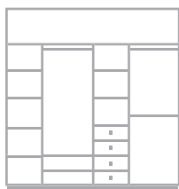
2 Door – 2400mm H x 2400mm W
